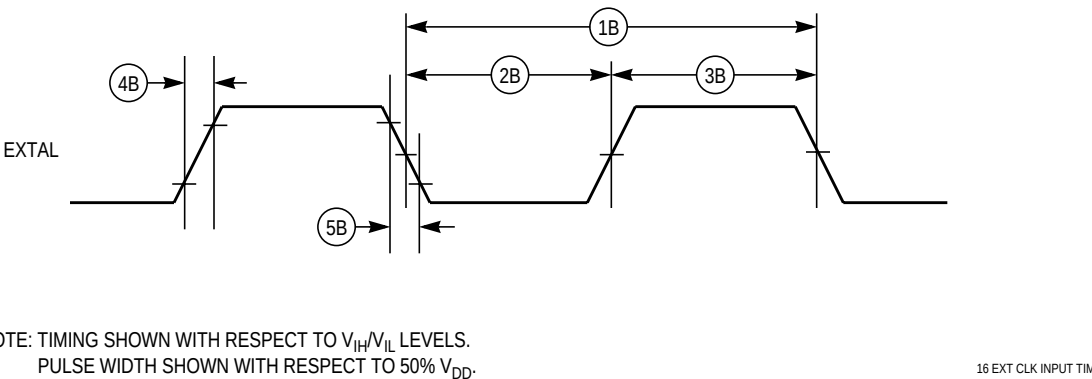
Figure A-2 External Clock Input Timing Diagram
