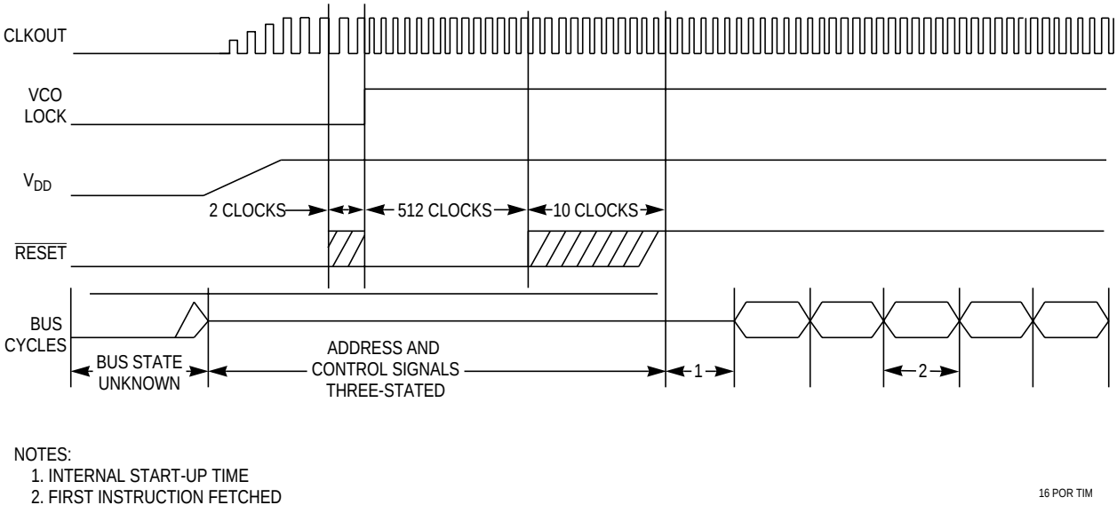
Figure 5-20 Power-On Reset
